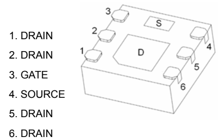
DFNWB2×2-6L-J
